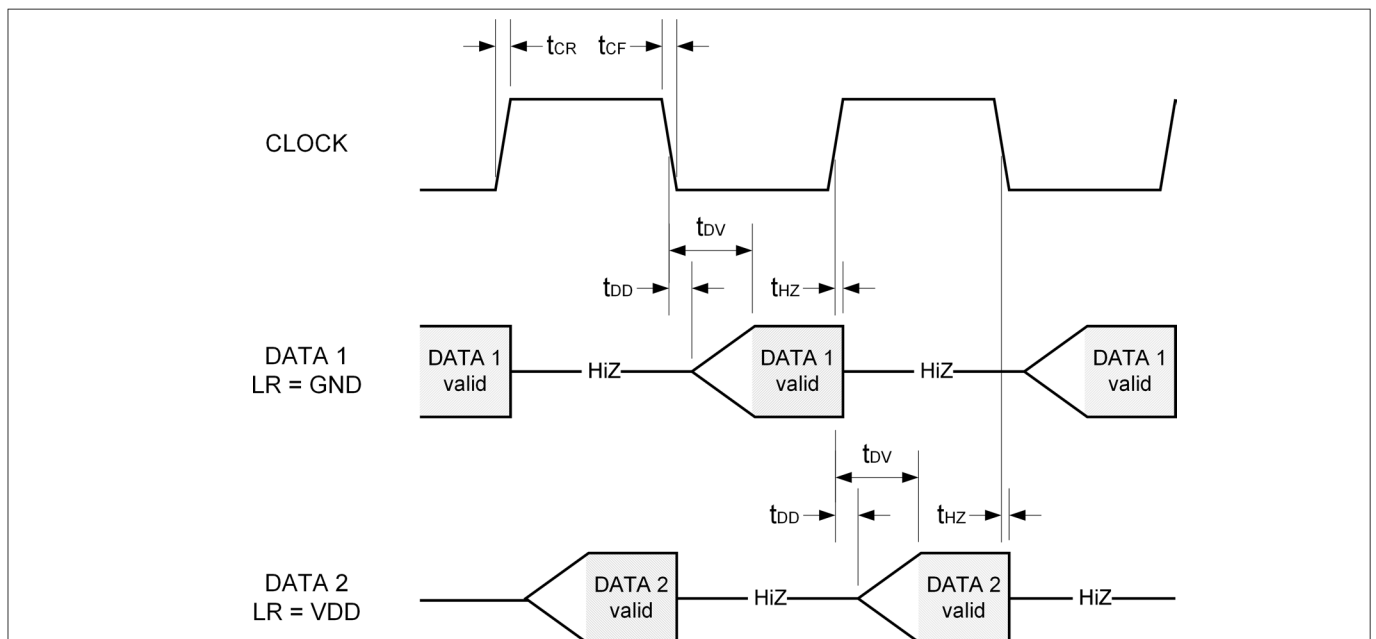
Figure 10 Timing diagram
