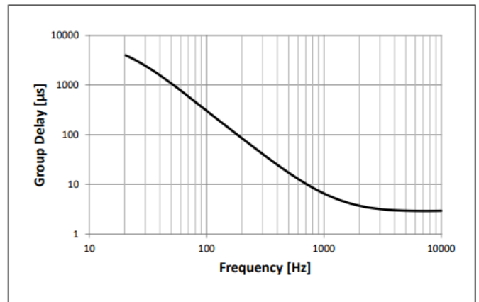
Figure 5 Typical group delay
