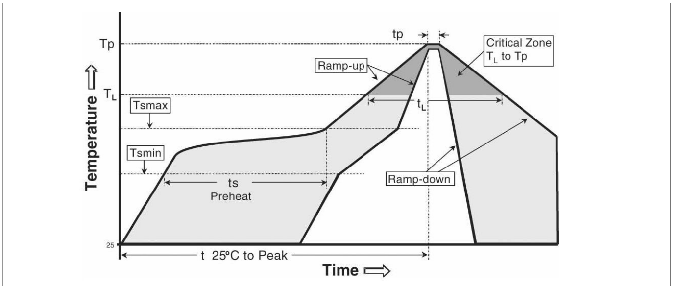
Figure 15 Recommended reflow
