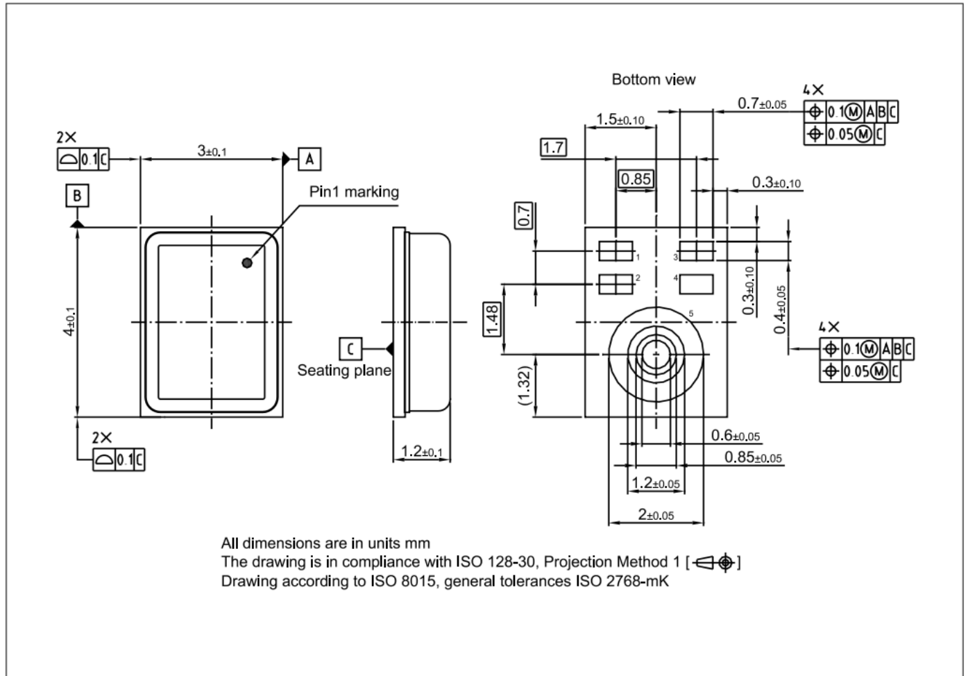
Figure 12 IM72D128V01 package drawing
