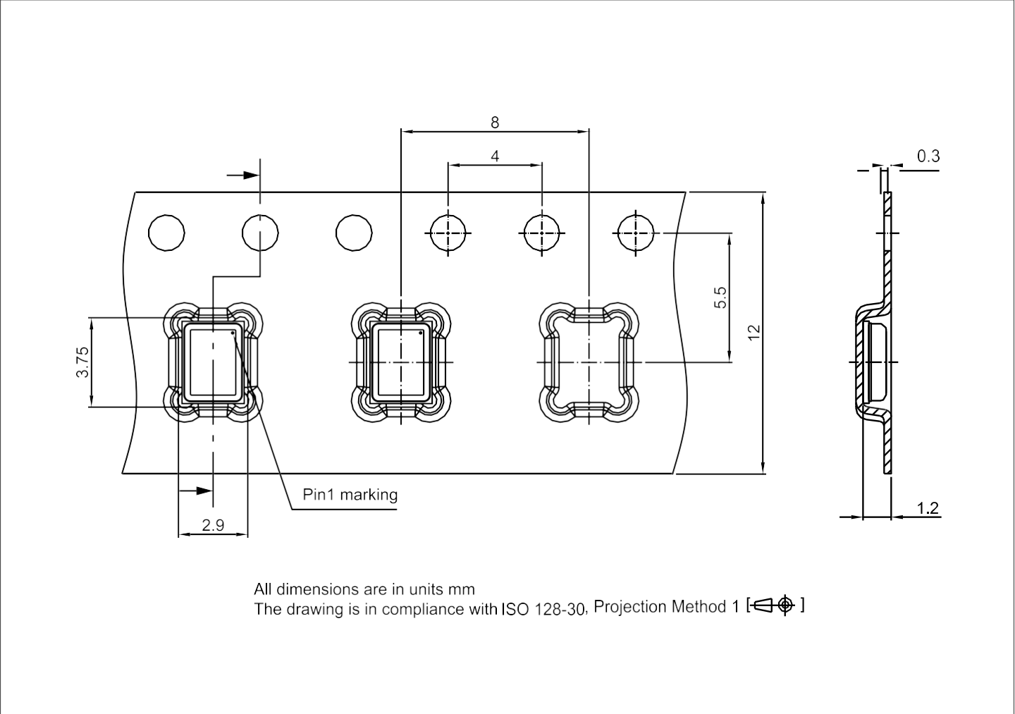
Figure 15 IM70D122V01 tape and reel packing
