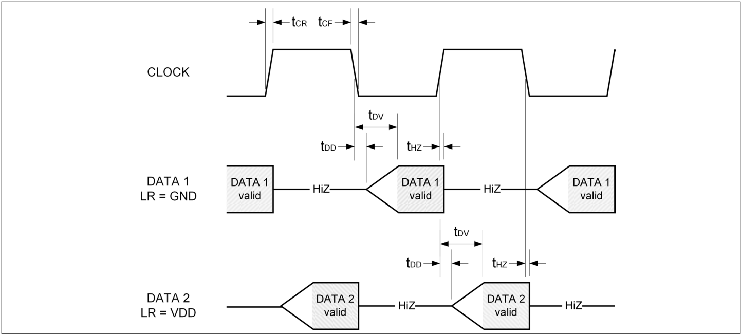
Figure 11 Timing diagram
