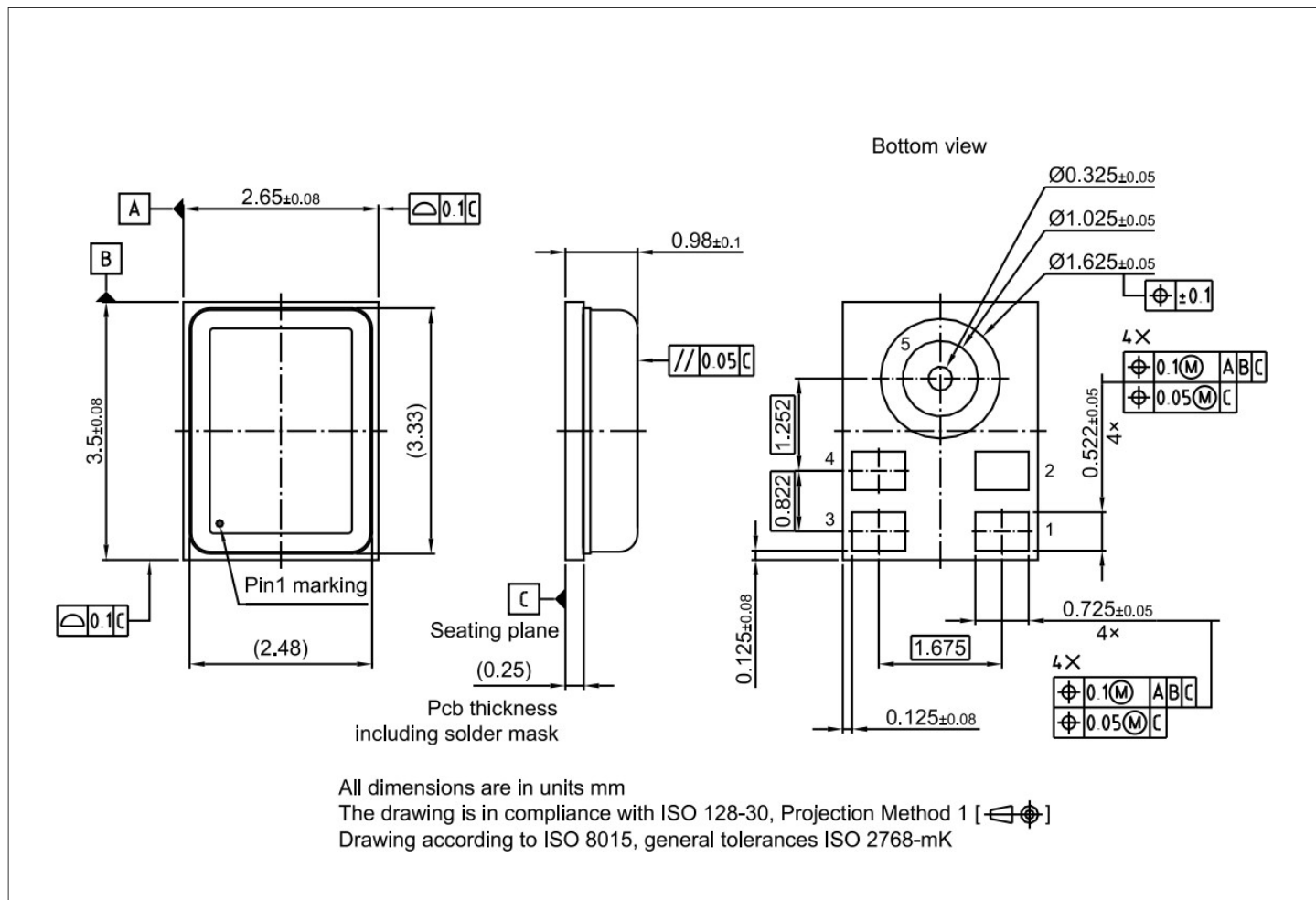
Figure 13 IM70D122V01 package
