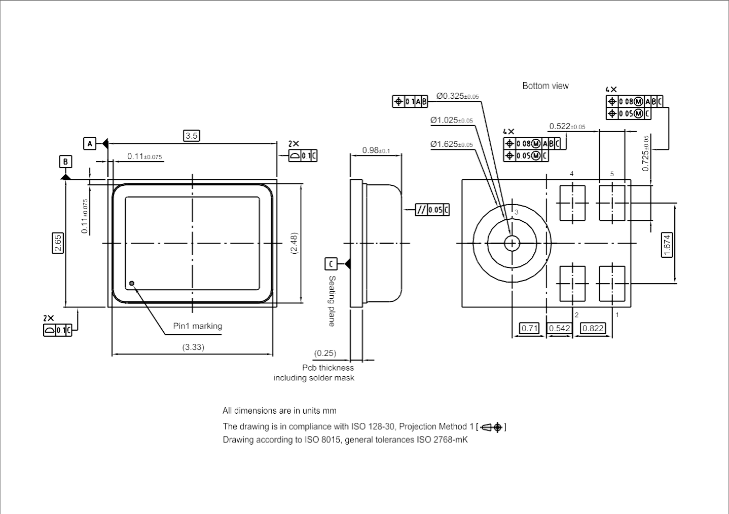
Figure 13 IM68D121JV01 package
