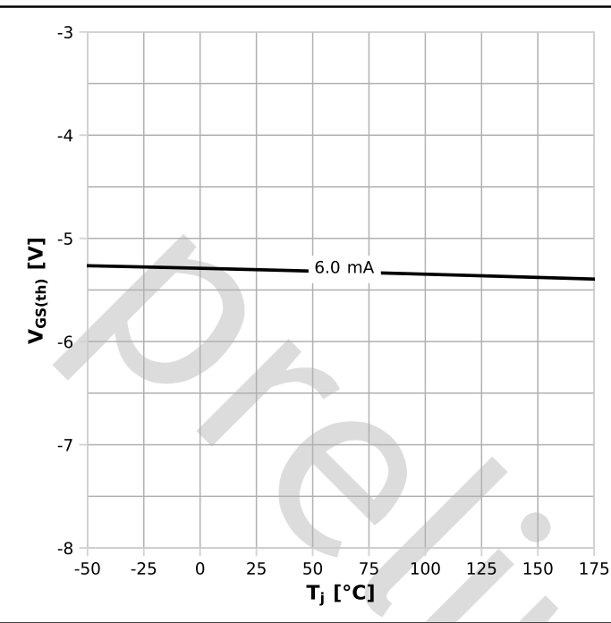
Diagram 15: Typ. gate threshold voltage
