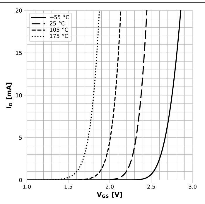
Diagram 16: Typ. transfer gate forward current
