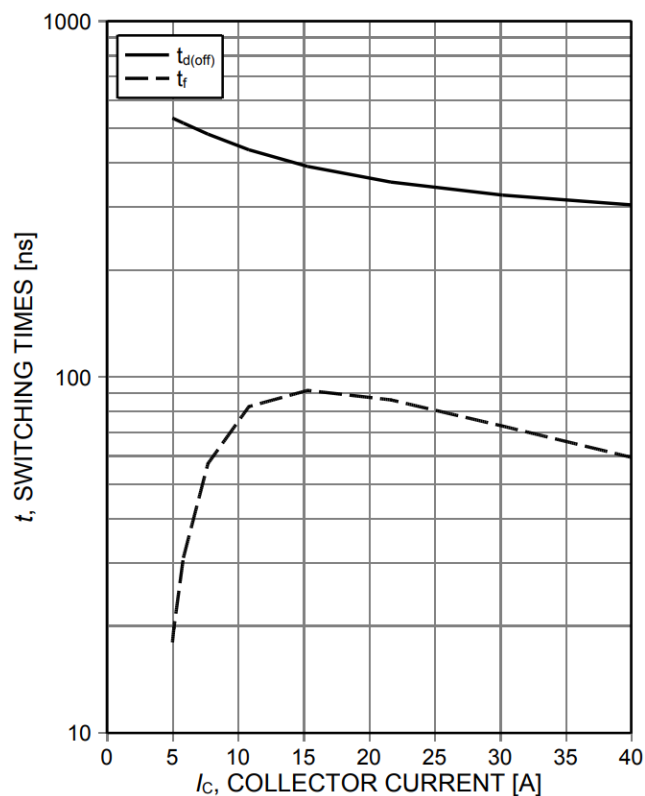
Figure 8. Typical switching times as a function of collector current (inductive load, T_j=175^\circ\text{C} , V_{CE}=600\text{V} , V_{GE}=0/15\text{V} , R_{G(on)}=10\Omega , R_{G(off)}=10\Omega , dynamic test circuit in Figure E)
