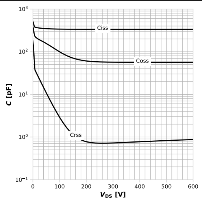
Diagram 18: Typ. capacitances
