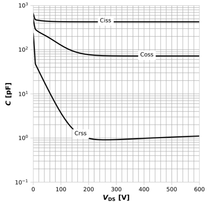
Diagram 18: Typ. capacitances
