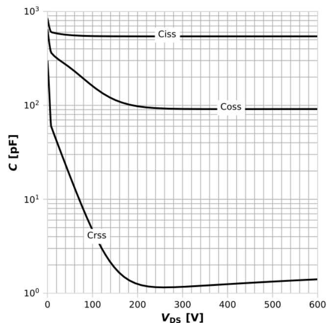
Diagram 18: Typ. capacitances
