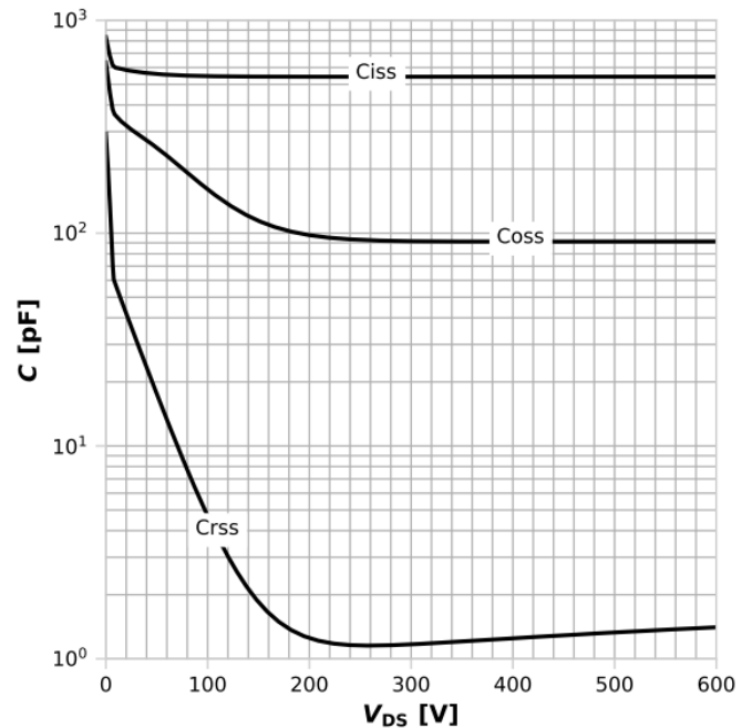
Diagram 18: Typ. capacitances
