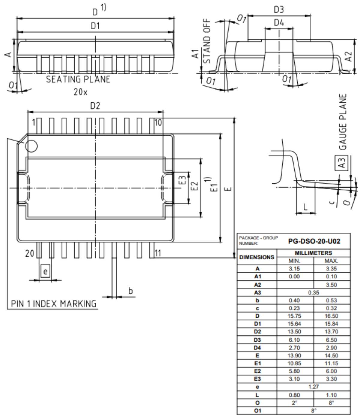
1) DOES NOT INCLUDE PLASTIC OR METAL PRUTRUSION OF 0.15 MAX. PER SIDE 图 1 PG-DSO- 20 外形图，尺寸单位为毫米
