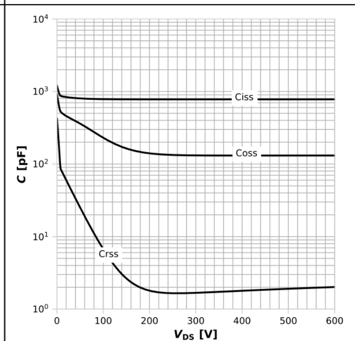
Diagram 18: Typ. capacitances
