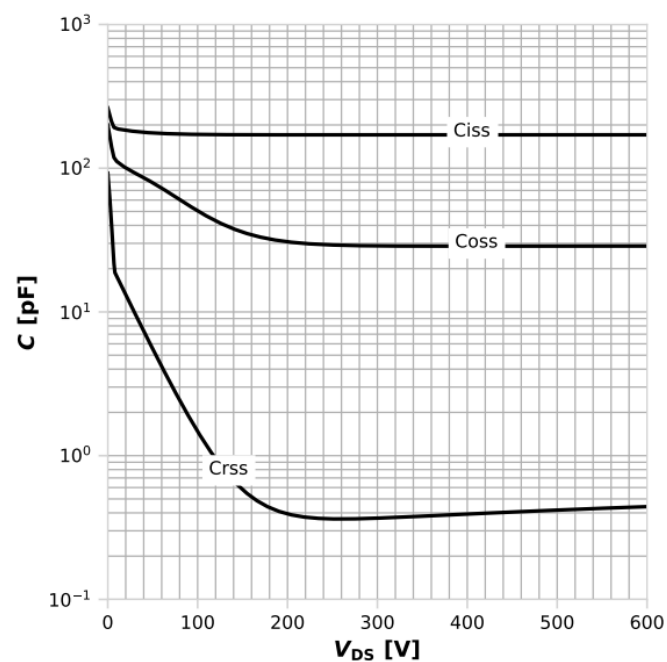
Diagram 18: Typ. capacitances
