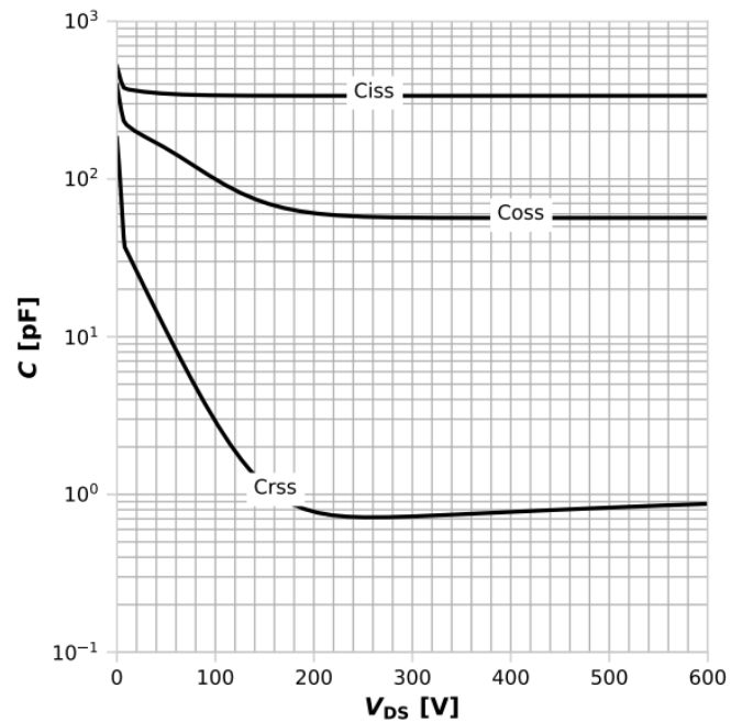
Diagram 18: Typ. capacitances
