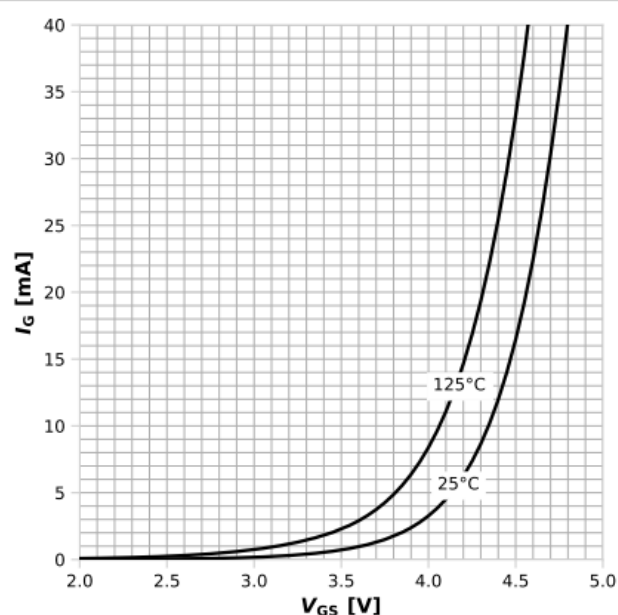
Diagram 14: Typ. transfer gate current characteristic
