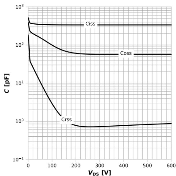
Diagram 18: Typ. capacitances
