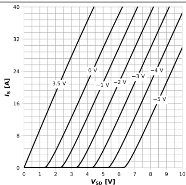
Diagram 16: Typ. channel reverse characteristics
