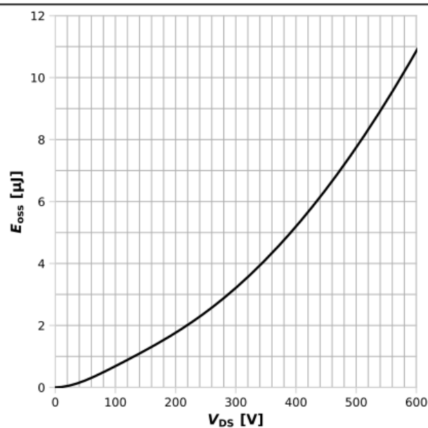
Diagram 20: Typ. Coss stored energy
