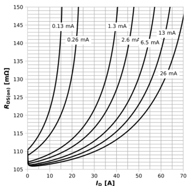
Diagram 9: Typ. Drain-source on-state resistance
