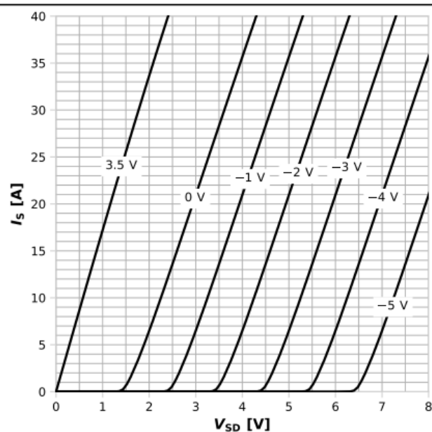
Diagram 15: Typ. channel reverse characteristics
