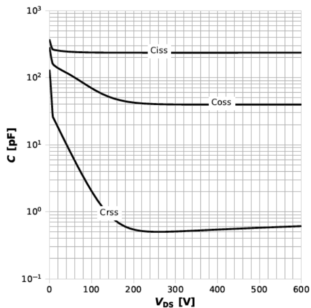
Diagram 18: Typ. capacitances
