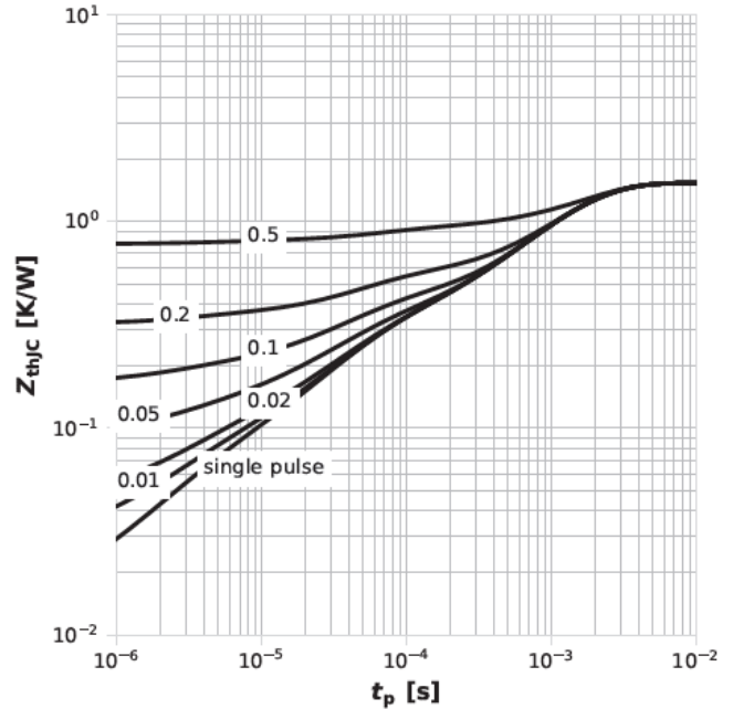
Diagram 2: Max. transient thermal impedance
