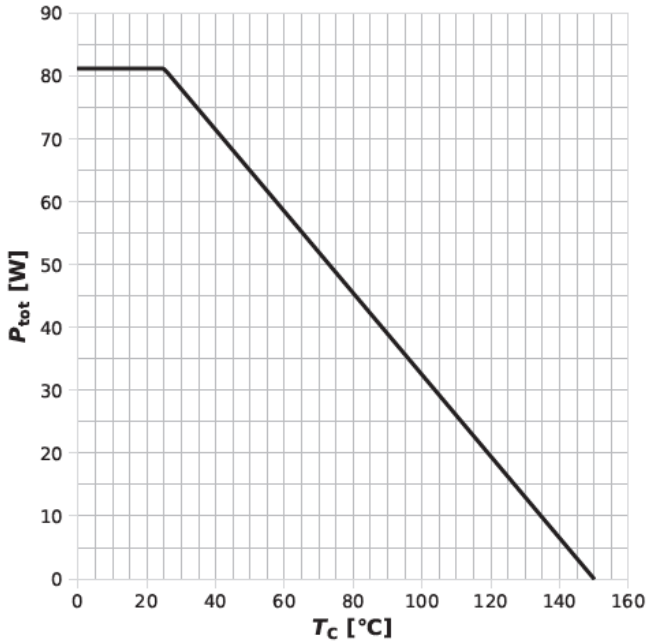
Diagram 1: Power dissipation
