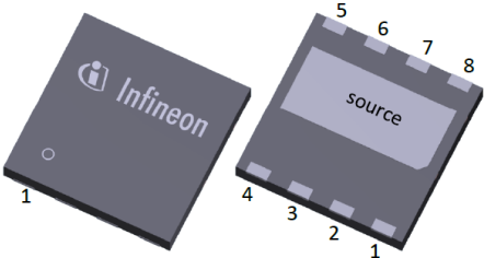
PG-TSON-8
