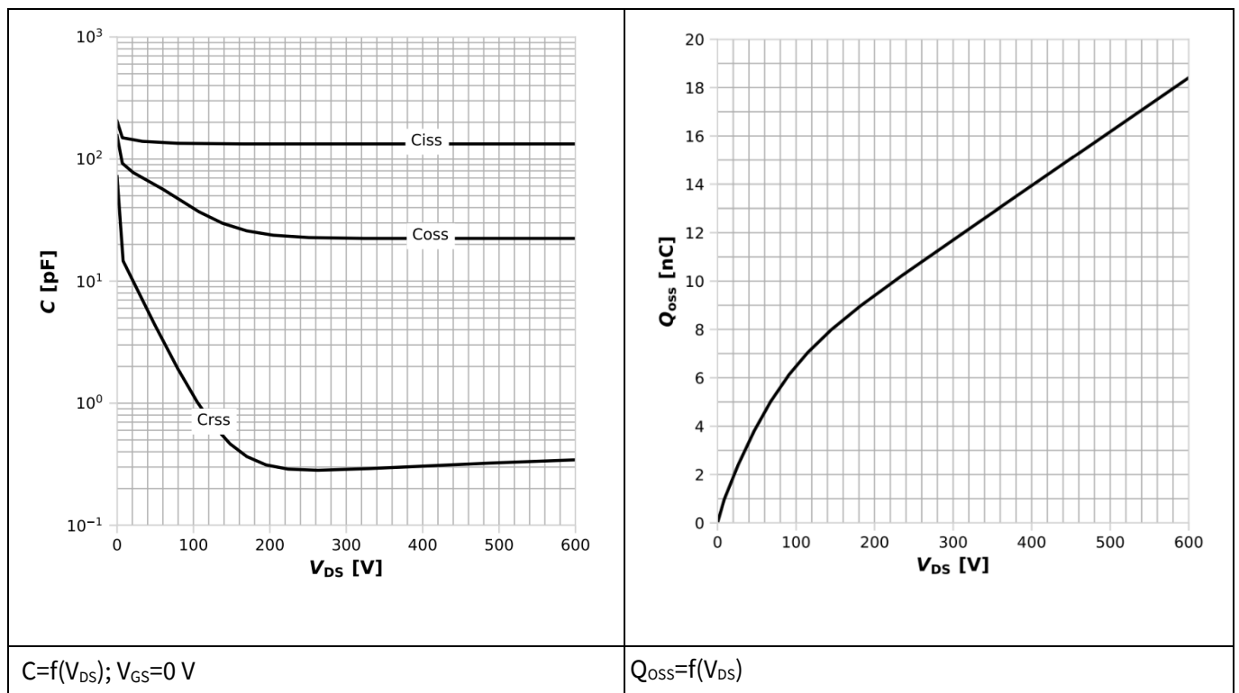
Figure 15 Terminal capacitances and output charge (single switch)
