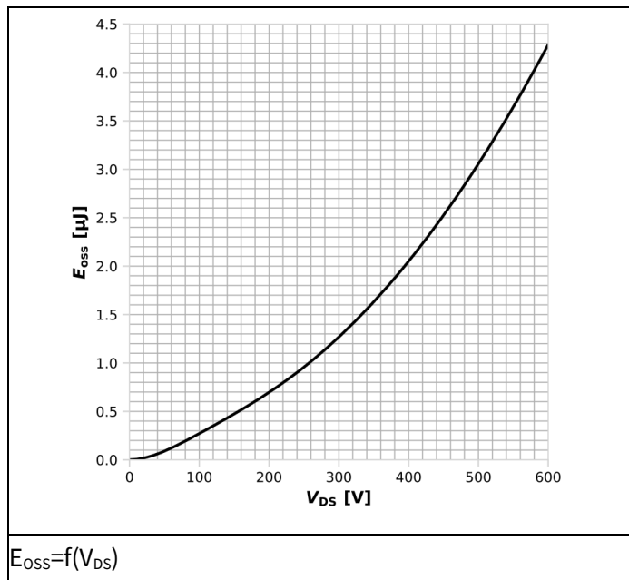
Figure 16 Typical output energy (single switch)
