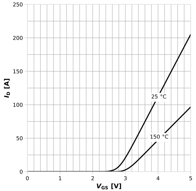
Diagram 6: Typ. transfer characteristics
