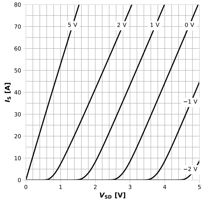
Diagram 8: Typ. channel reverse characteristics
