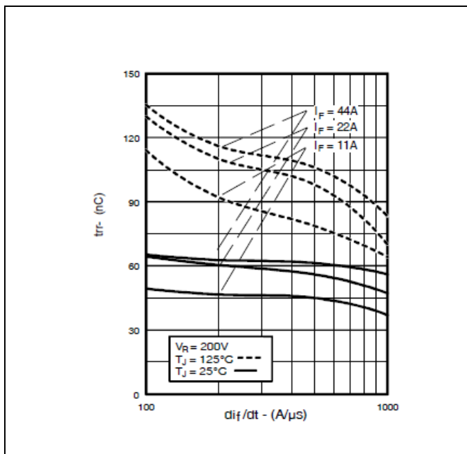
Figure 5 Typical Reverse Recovery Vs. di_i/dt
