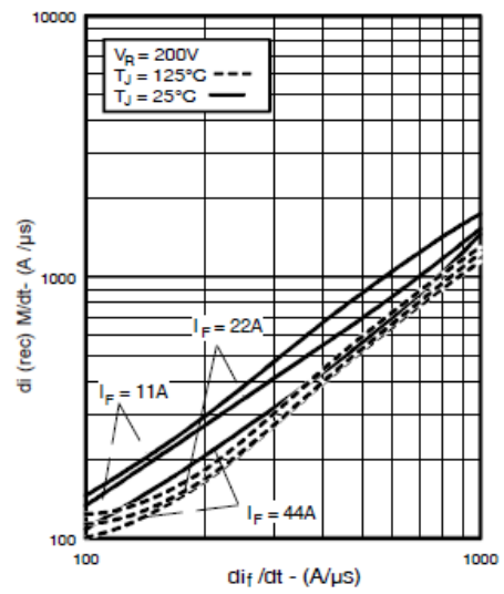
Figure 8 Typical di_{(rec)M}/dt Vs. di_f/dt
