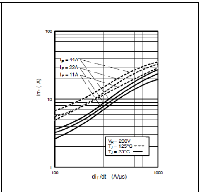
Figure 6 Typical Recovery Current Vs. di_i/dt
