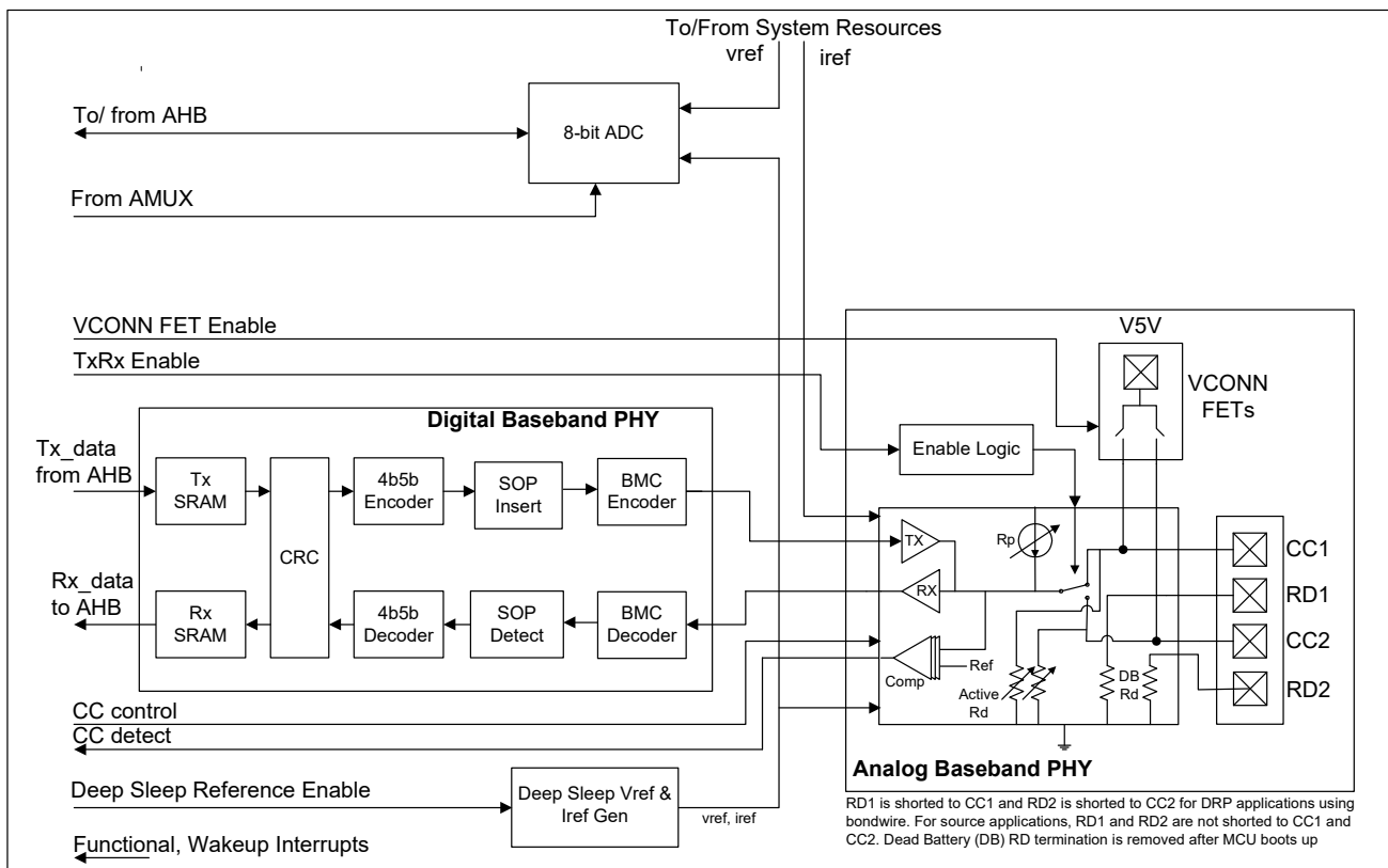
Figure 1. USB-PD Subsystem
