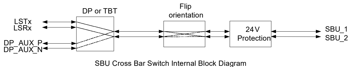
Figure 2. CCG6 SBU Crossbar Switch Block Diagram
