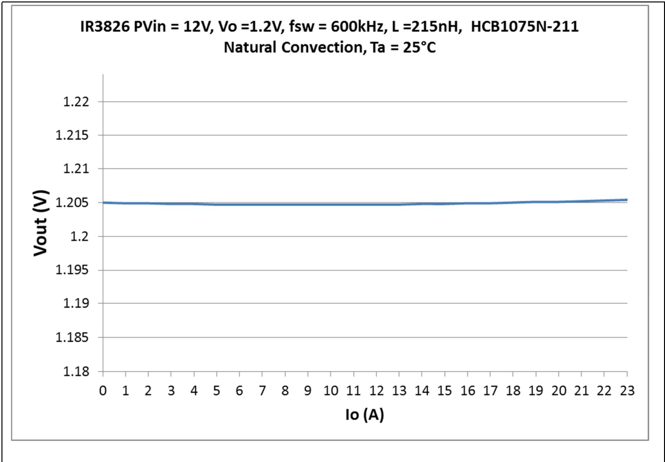
Figure 20 Load regulation
