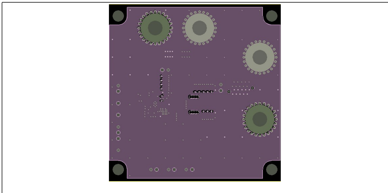
Figure 4 Mid layer 1
