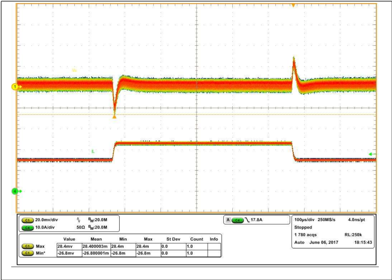
Figure 17 Transient response at 8A step load current @ 2.5 A/μs slew rate: I o = 15 A – 23 A, (Ch 1 : V o , Ch 4 : I o ), Undershoot: -26.8 mV, Overshoot: 28.4 mV
