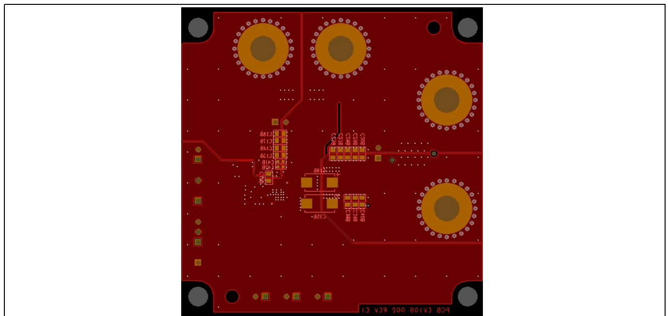
Figure 3 Bottom layer
