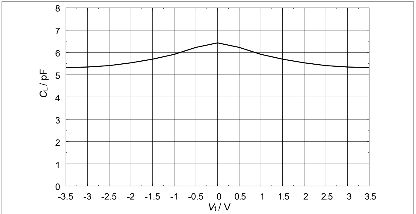
图4 结电容: C_L = f(V_t) , f = 1\text{ MHz}
