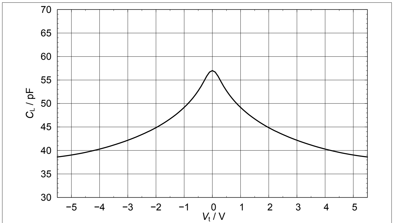
Figure 4 Line capacitance: C_L = f(V_t) , f = 1 MHz
