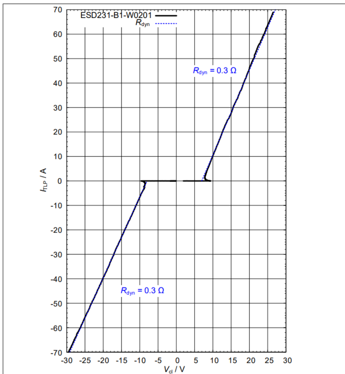
图9 钳位电压 (TLP): I_{TLP} = f(V_{cl})
