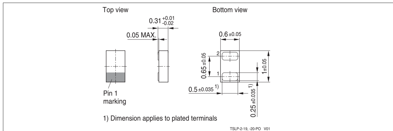
Figure 5-5 TSLP-2-19 Package outline
