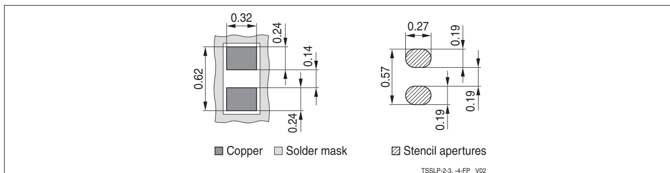
Figure 5-2 TSSLP-2-3 Footprint
