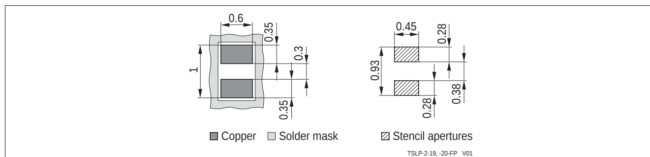
Figure 5-6 TSLP-2-19 Footprint
