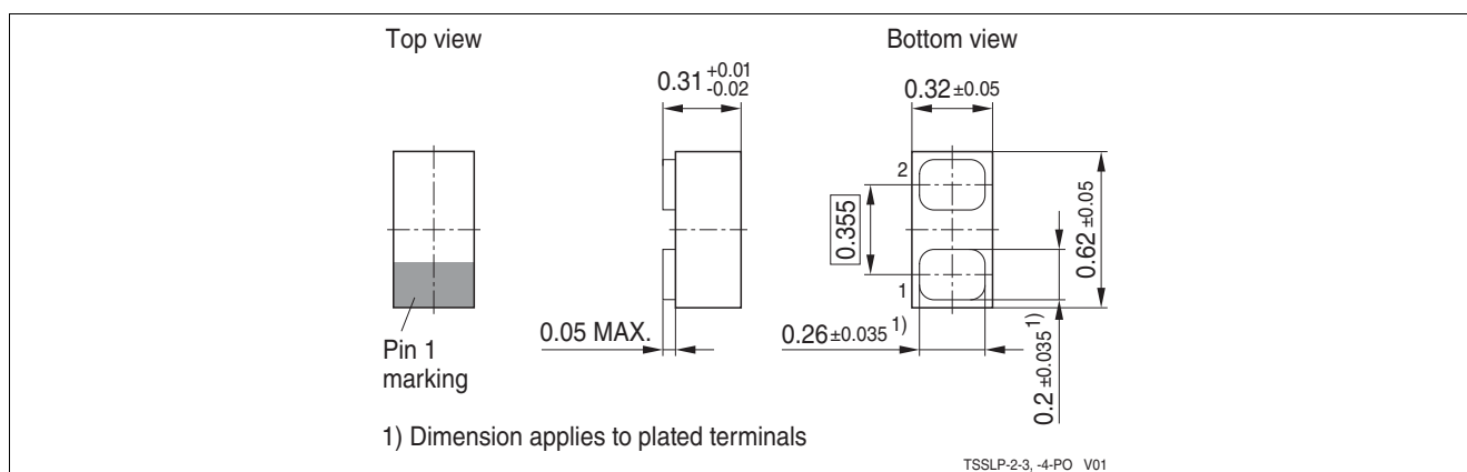
Figure 5-1 TSSLP-2-3 Package outline
