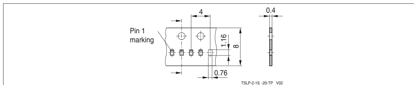
Figure 5-7 TSLP-2-19 Packing
