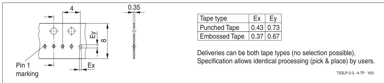
Figure 5-3 TSSLP-2-3 Packing
