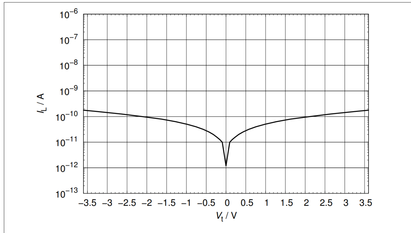
图3 漏电流: I_L = f(V_t)
