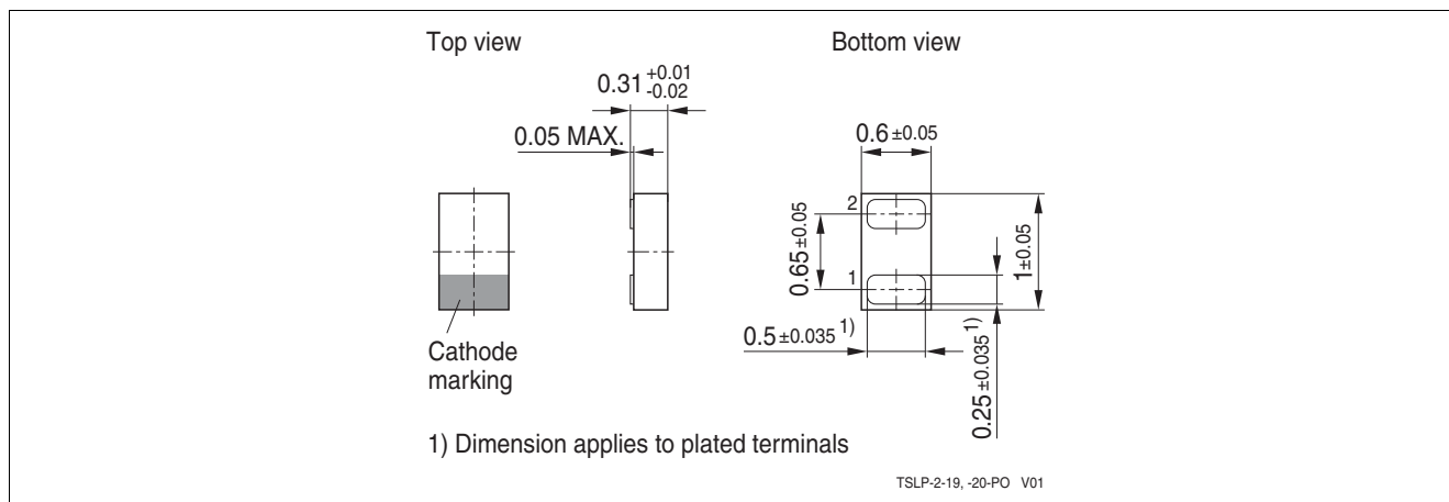
Figure 4-5 TSLP-2-20: Package overview
