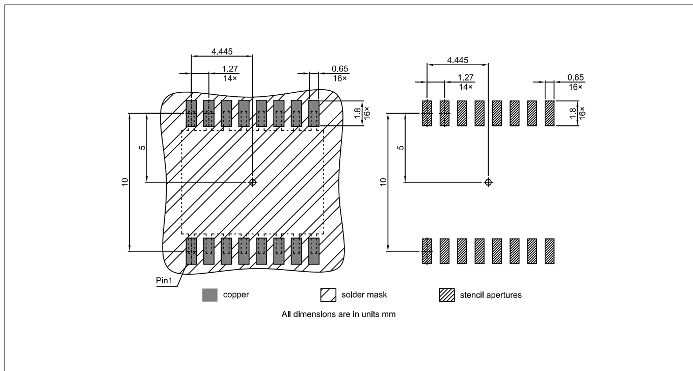
Figure 23 DSO16-300mil footprint
