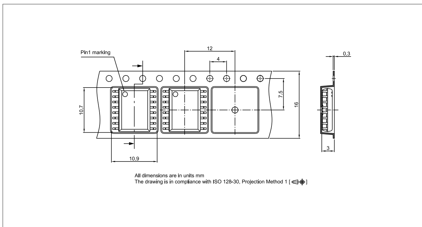
Figure 24 DSO16-300mil packing
