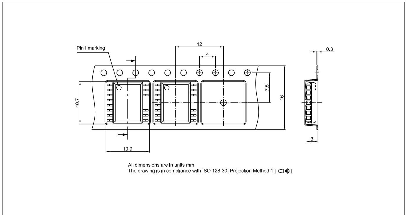
Figure 27 DSO14-300mil packing
