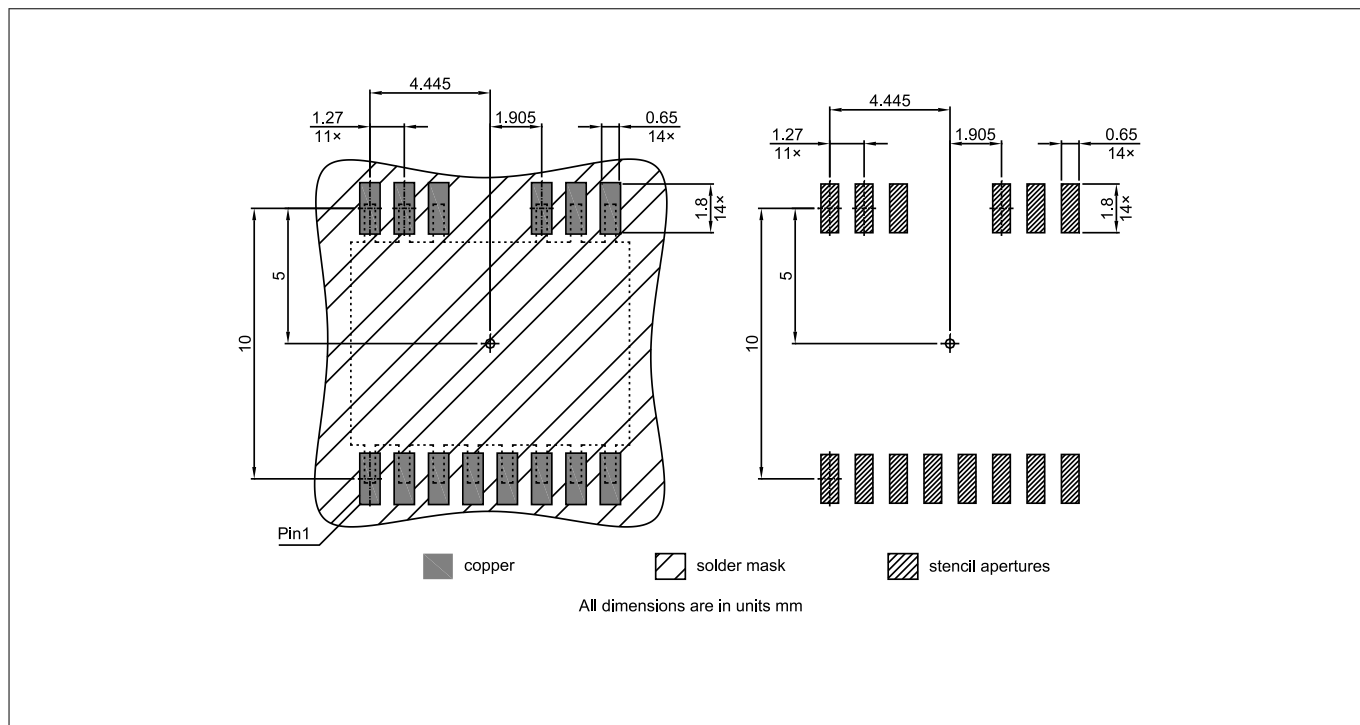
Figure 26 DSO14-300mil footprint
