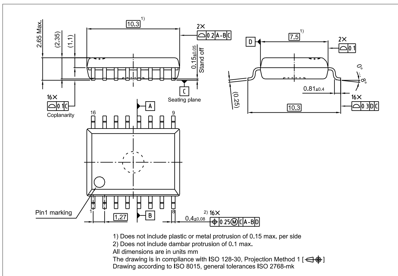
Figure 22 DSO16-300mil outline
