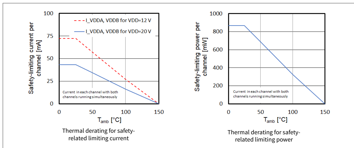
Figure 21 Thermal derating curves
