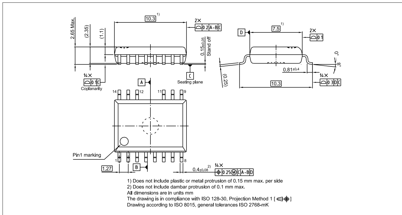
Figure 25 DSO14-300mil outline
