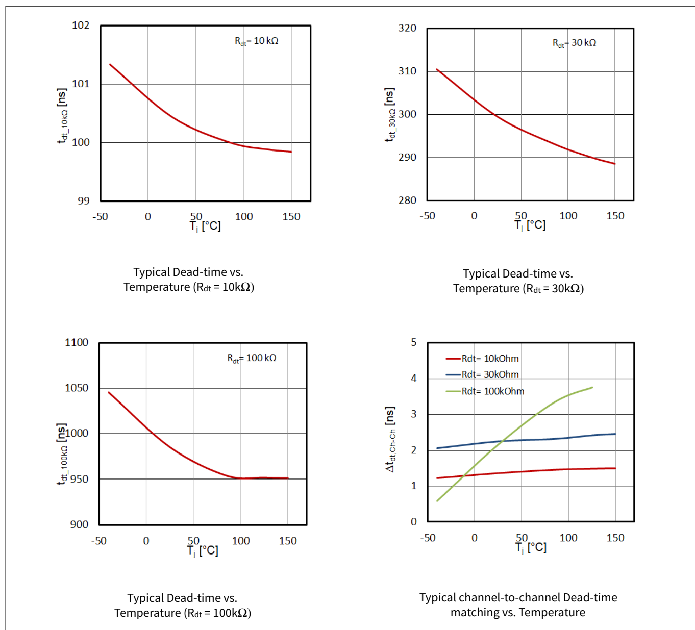
Figure 20 Typical Dead-time
