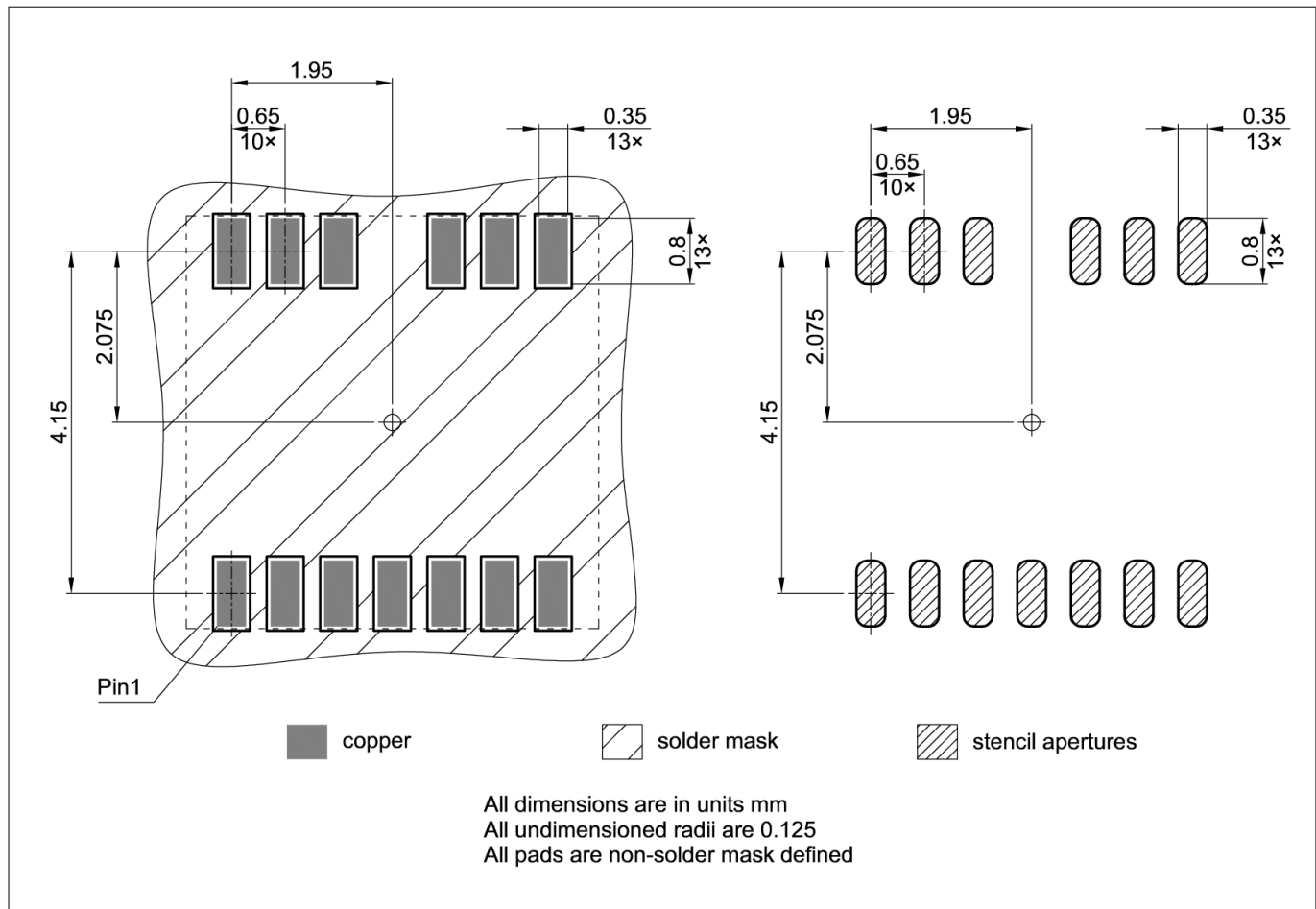
Figure 22 LGA5x5 footprint
