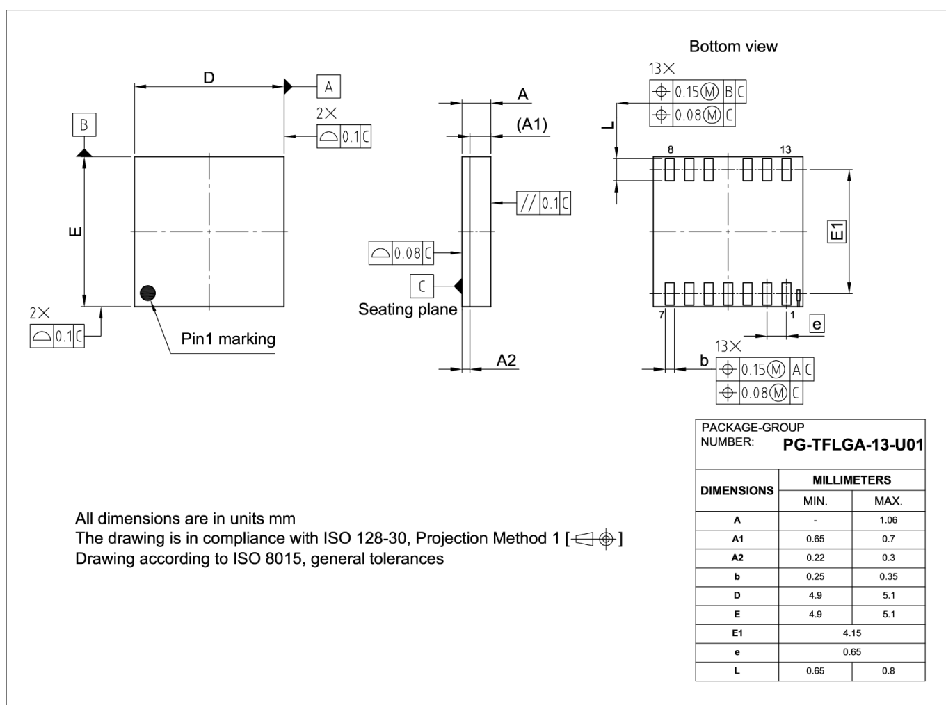
Figure 21 LGA 5x5 package outline
