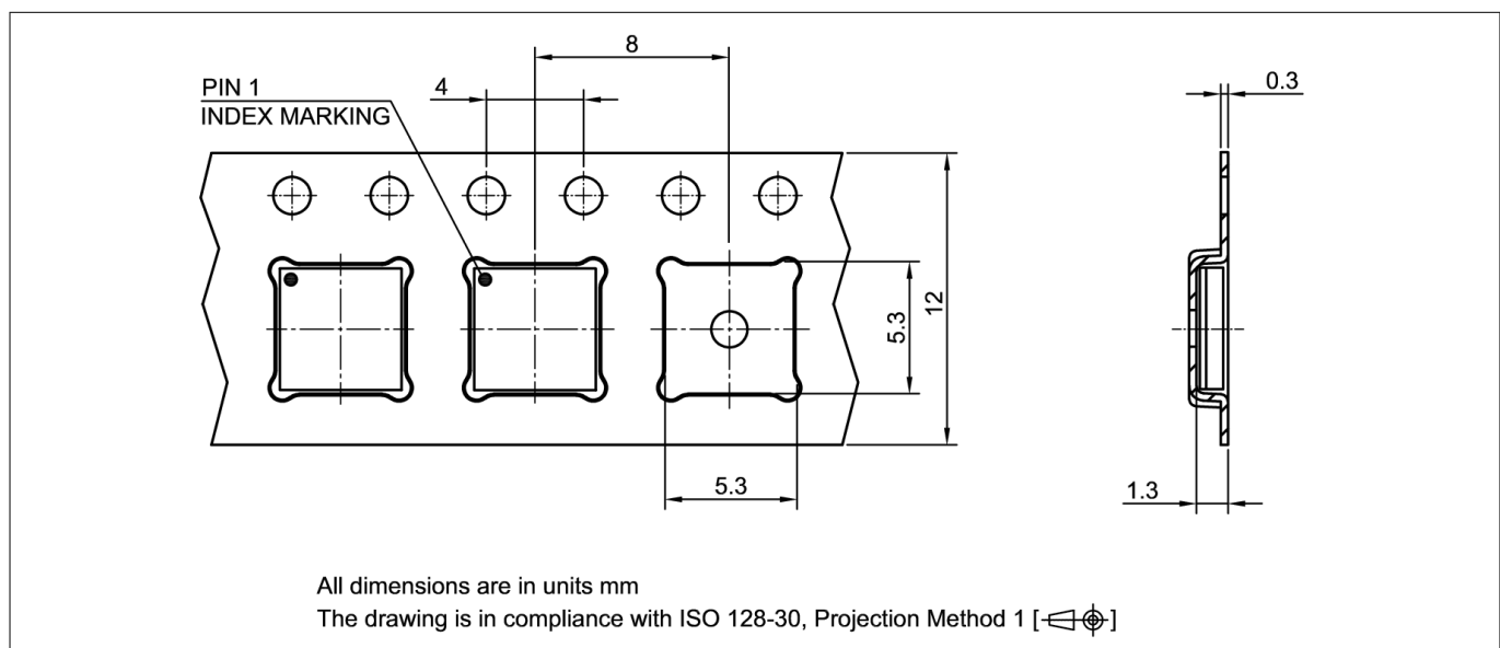
Figure 23 LGA5x5 packing
