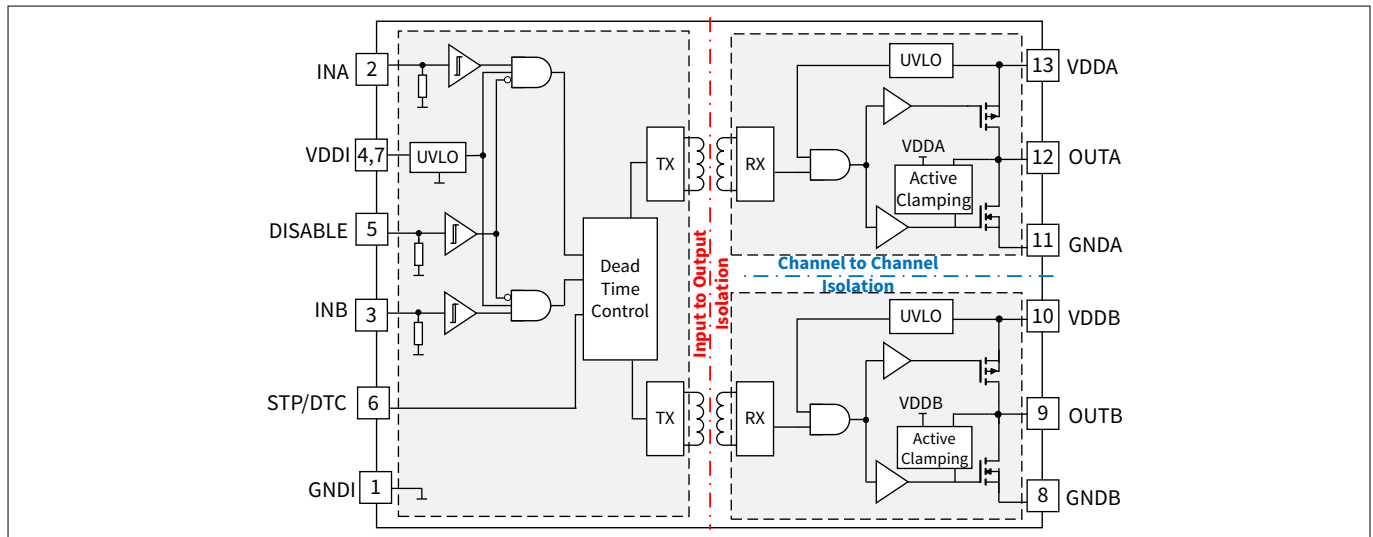
Figure 3 Block diagram
