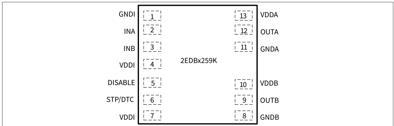
Figure 2 Pin configuration (top side view)
