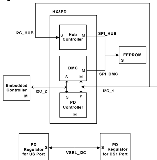
Figure 4. Communication Interfaces
