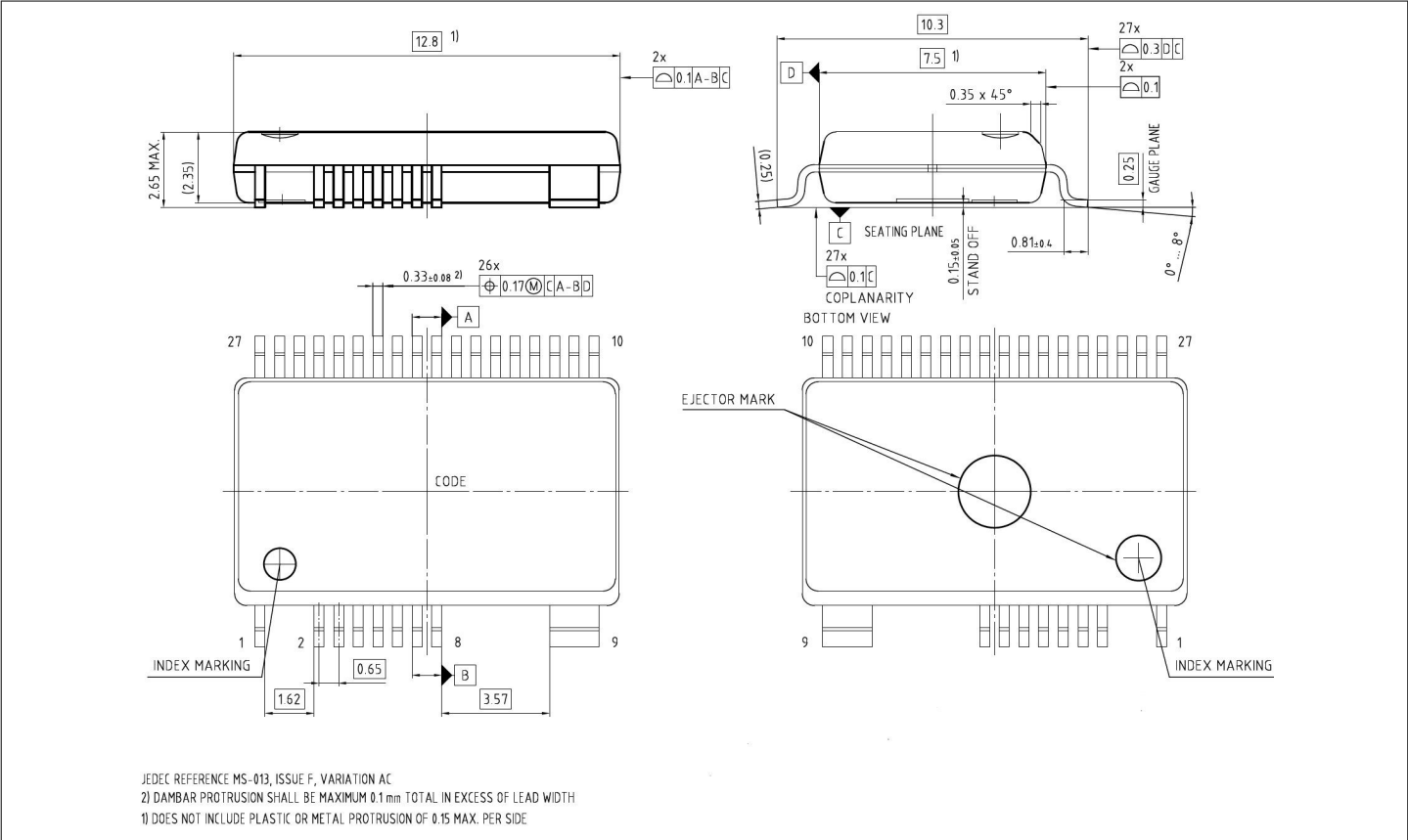
Figure 10 Outline dimensions PG-DSO-27-1
