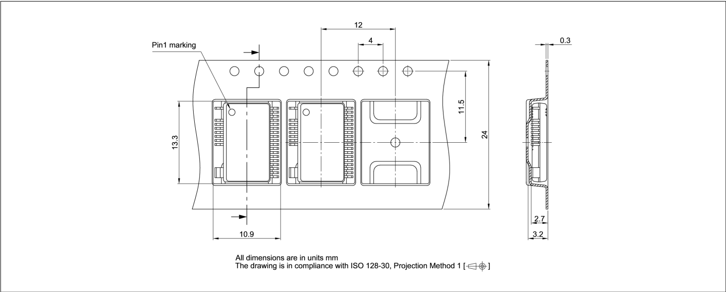
Figure 13 Packaging PG-DSO-27-1
