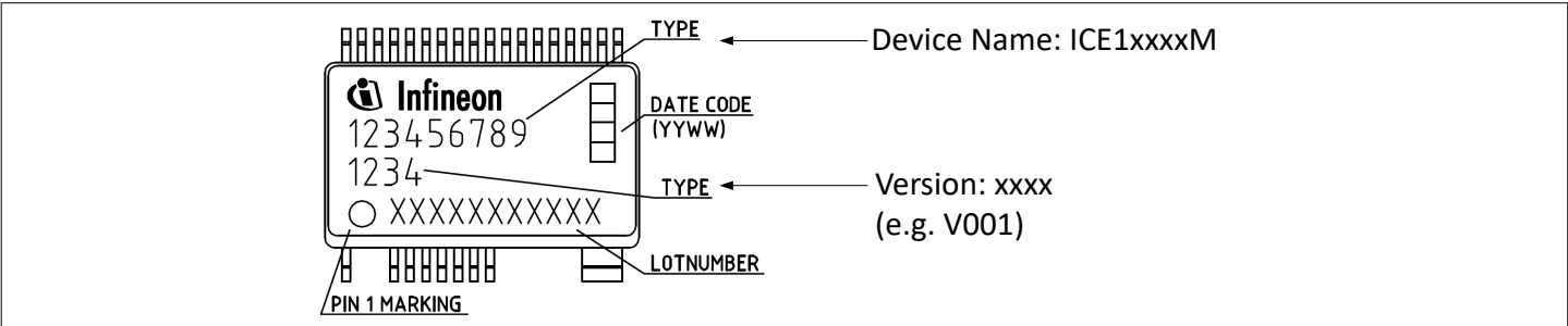
Figure 12 Marking PG-DSO-27-1
