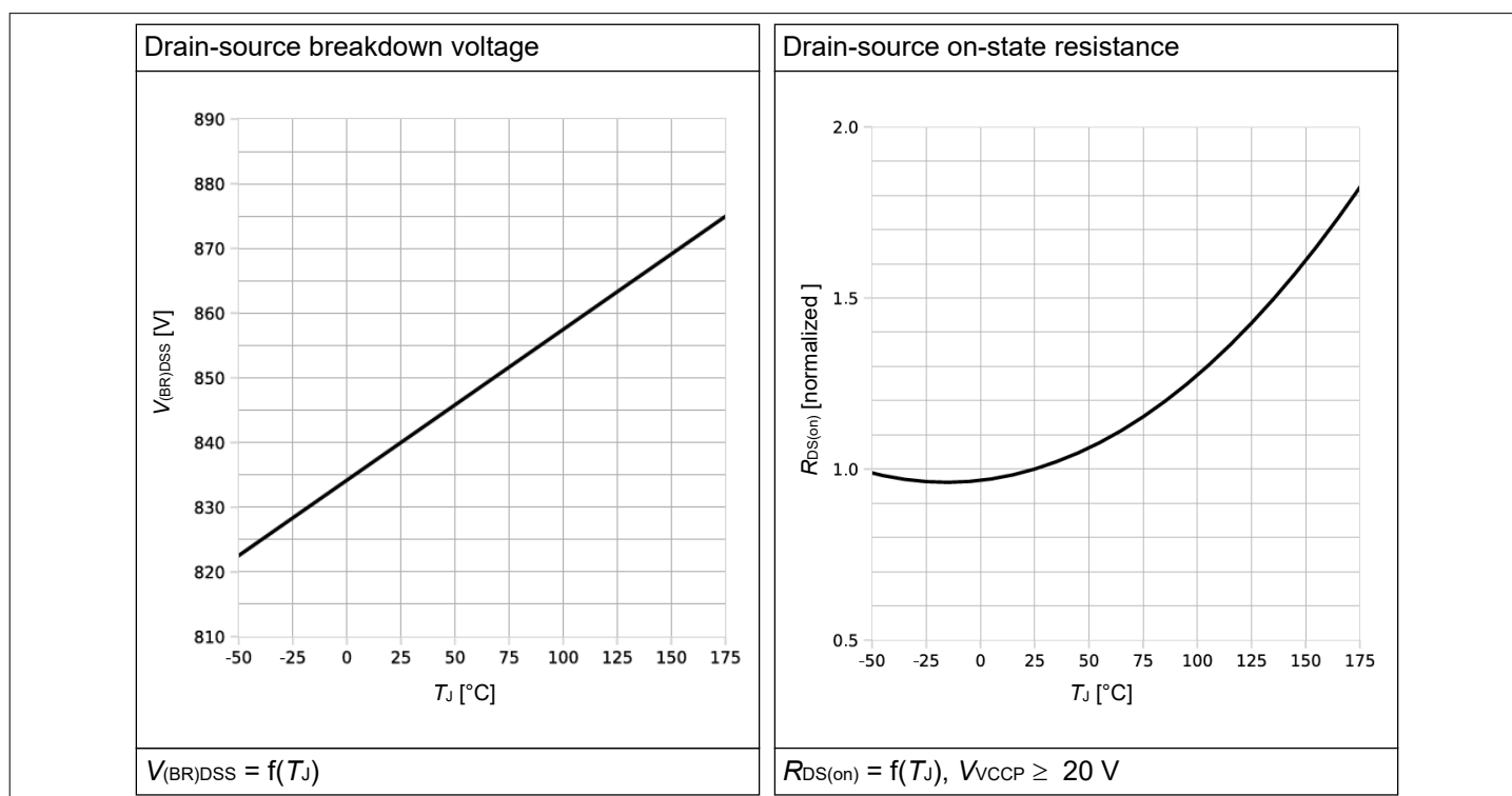
Figure 9 Breakdown voltage and R_{ds(on)} over temperature
