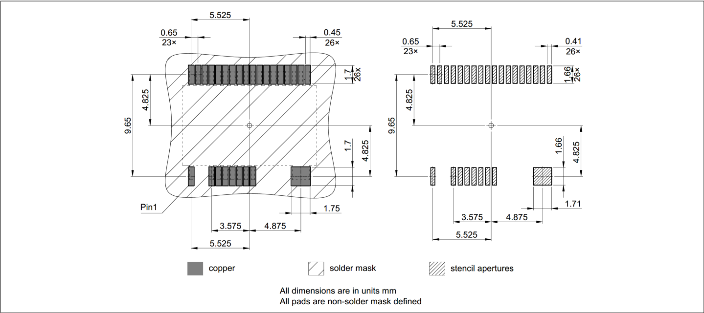
Figure 11 Footprint PG-DSO-21-1
