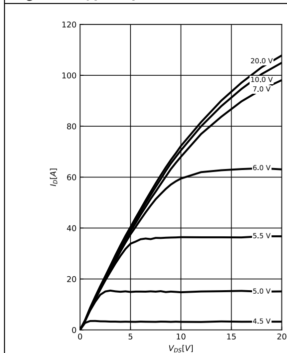
Diagram 3: Typ. output characteristics
