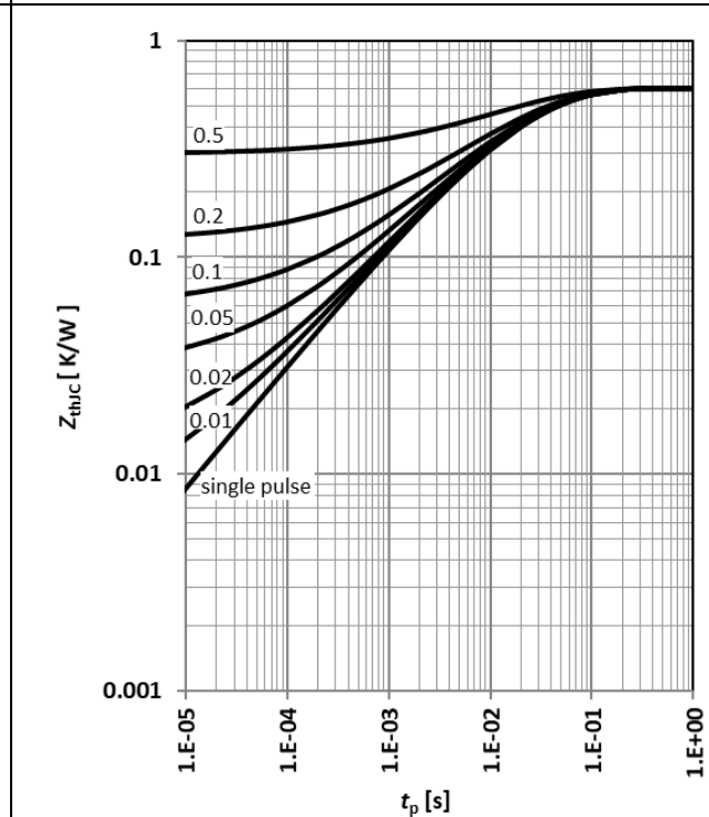
Diagram 2: Max. transient thermal impedance
