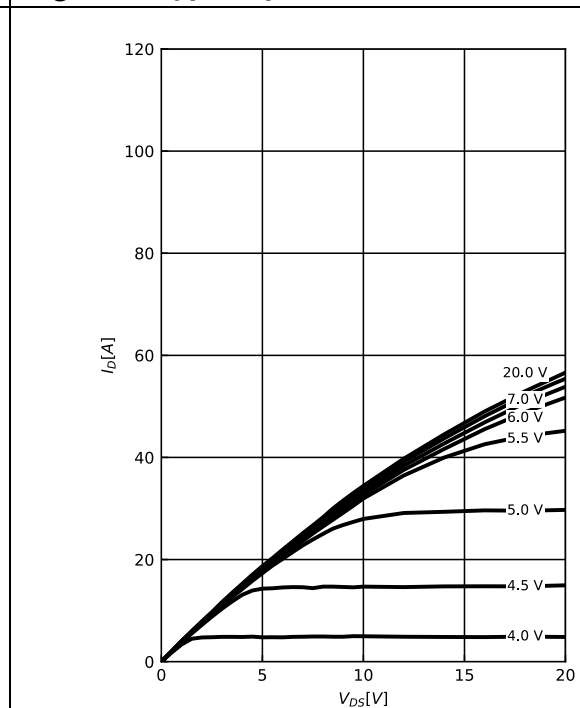
Diagram 4: Typ. output characteristics
