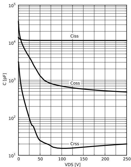
Diagram 11: Typ. capacitances
