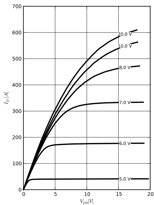
Diagram 3: Typ. output characteristics
