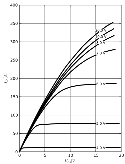
Diagram 4: Typ. output characteristics
