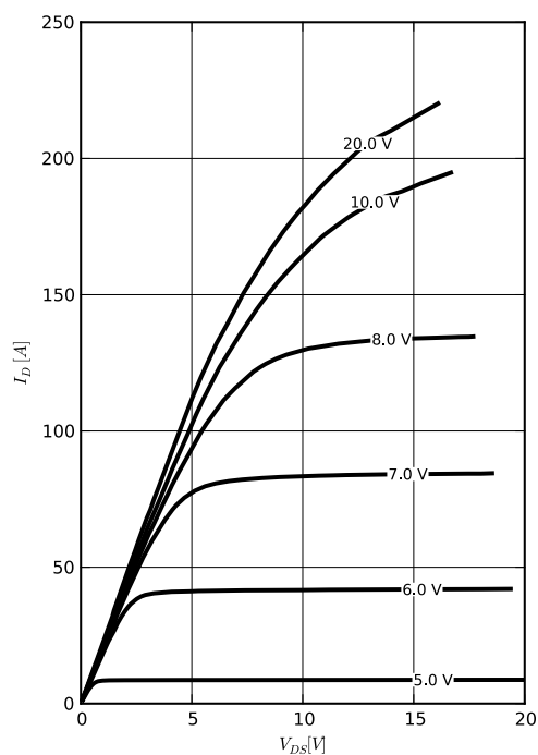
Diagram 3: Typ. output characteristics
