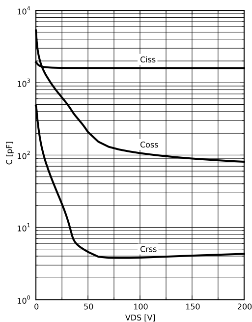
Diagram 11: Typ. capacitances
