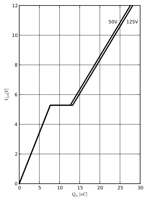
Diagram 12: Typ. gate charge
