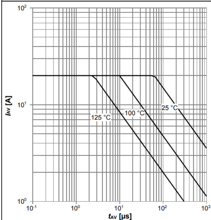
Diagram 13: Avalanche characteristics
