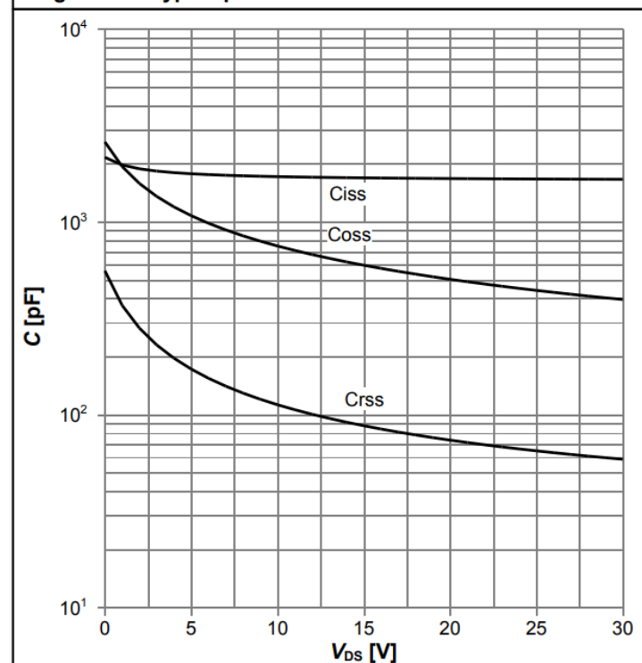
Diagram 11: Typ. capacitances
