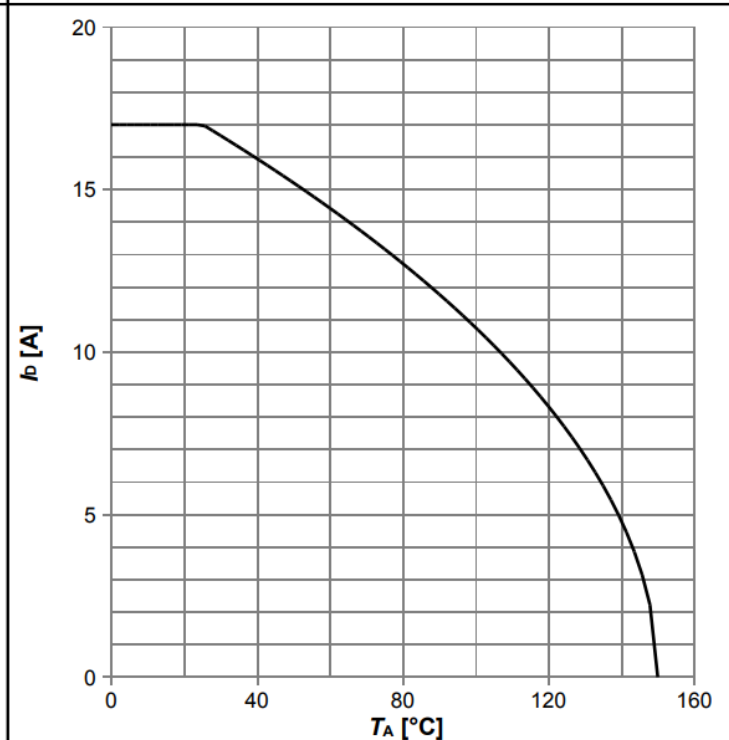
Diagram 2: Drain current
