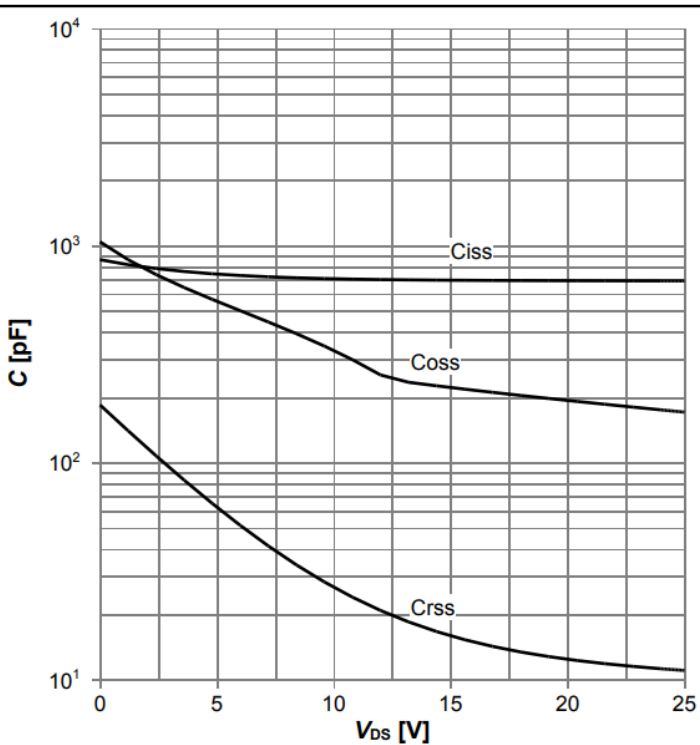
Diagram 11: Typ. capacitances
