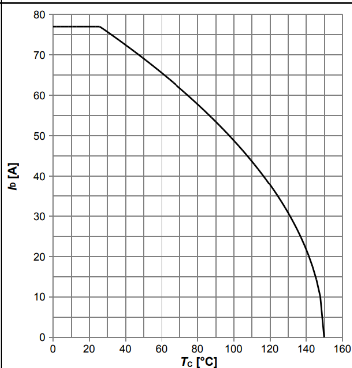
Diagram 2: Drain current
