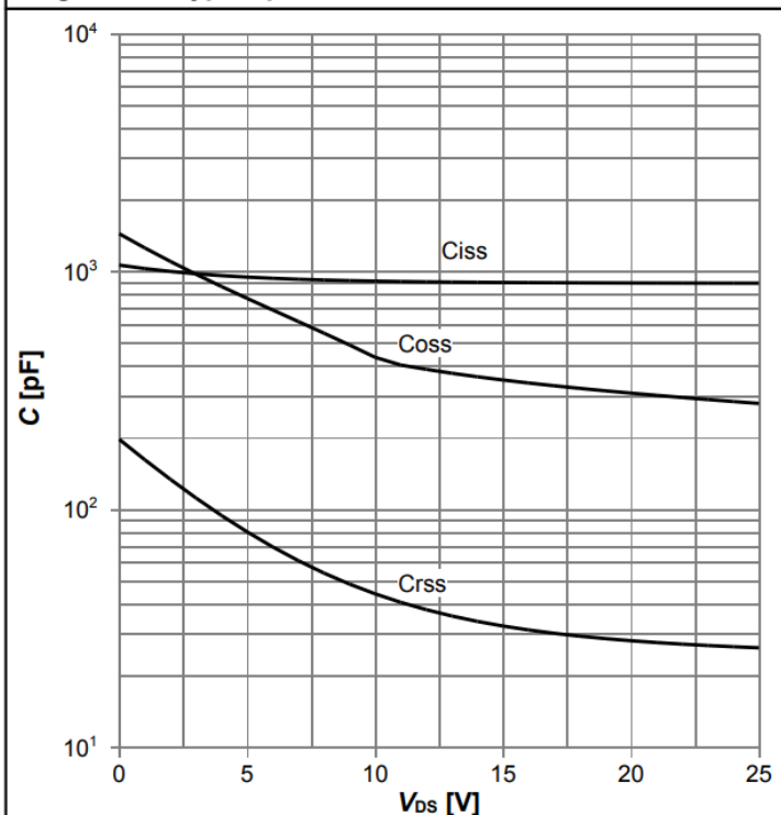
Diagram 11: Typ. capacitances
