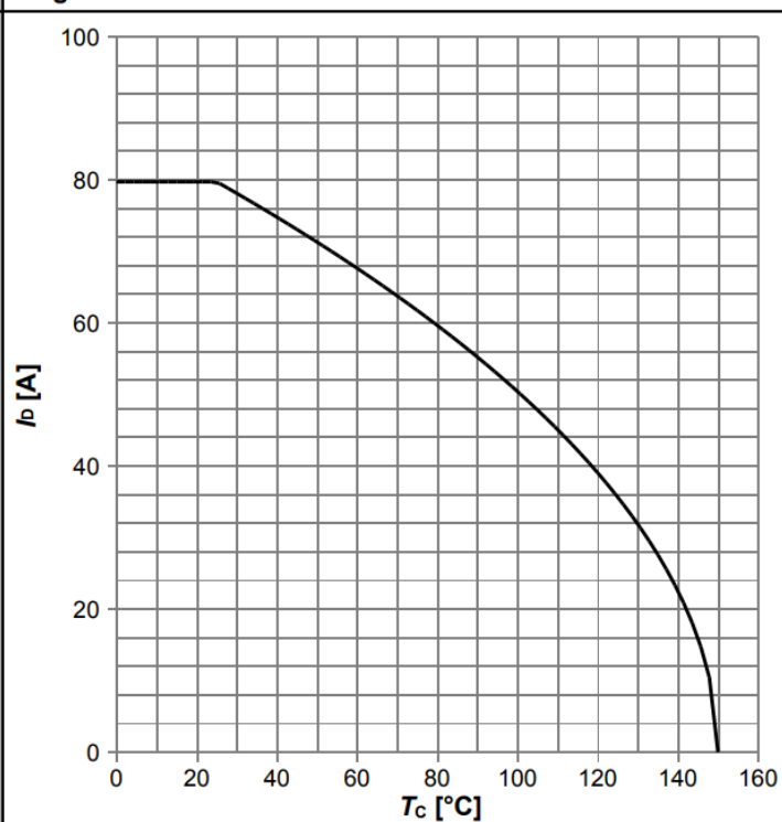
Diagram 2: Drain current
