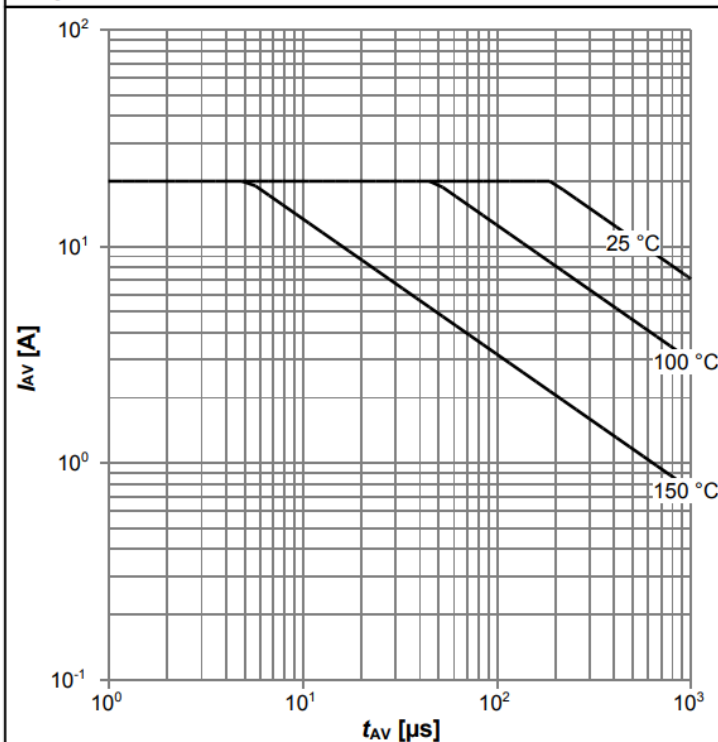
Diagram 13: Avalanche characteristics
