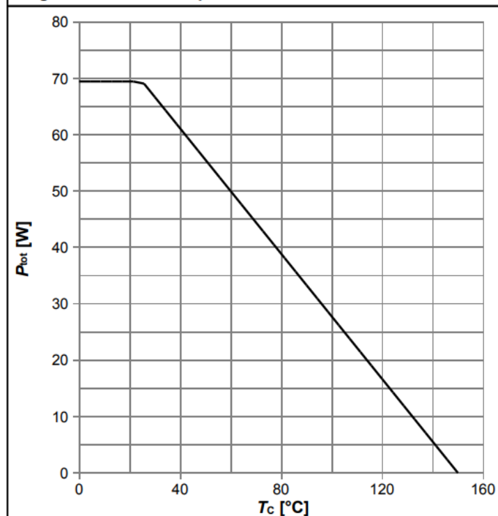
Diagram 1: Power dissipation
