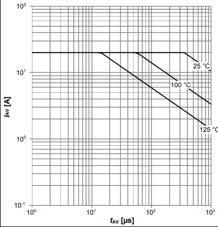
Diagram 13: Avalanche characteristics
