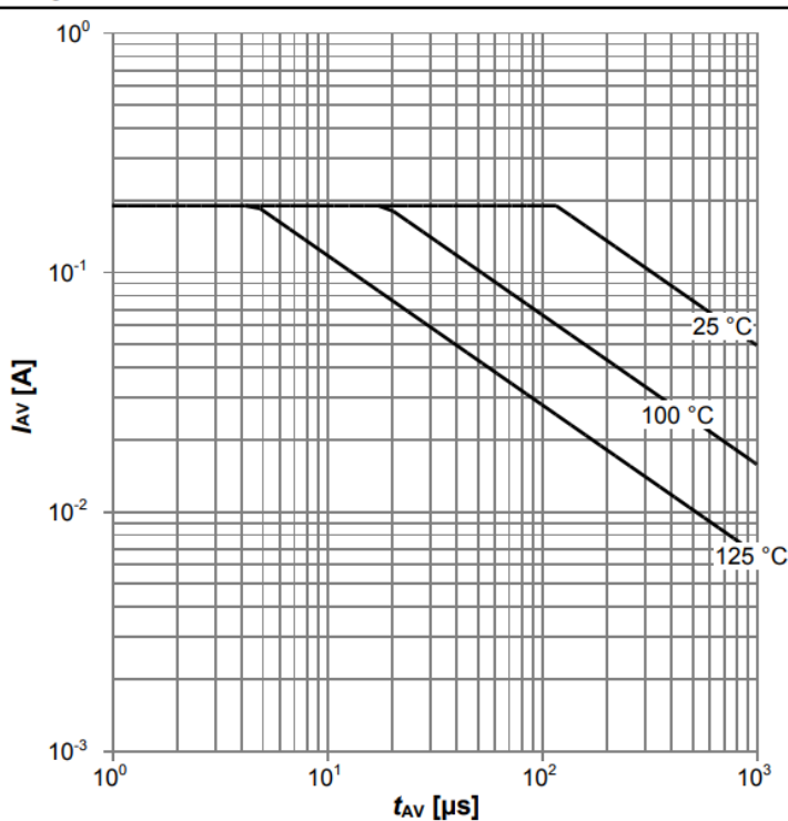
Diagram 13: Avalanche characteristics
