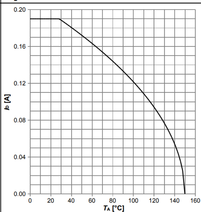
Diagram 2: Drain current
