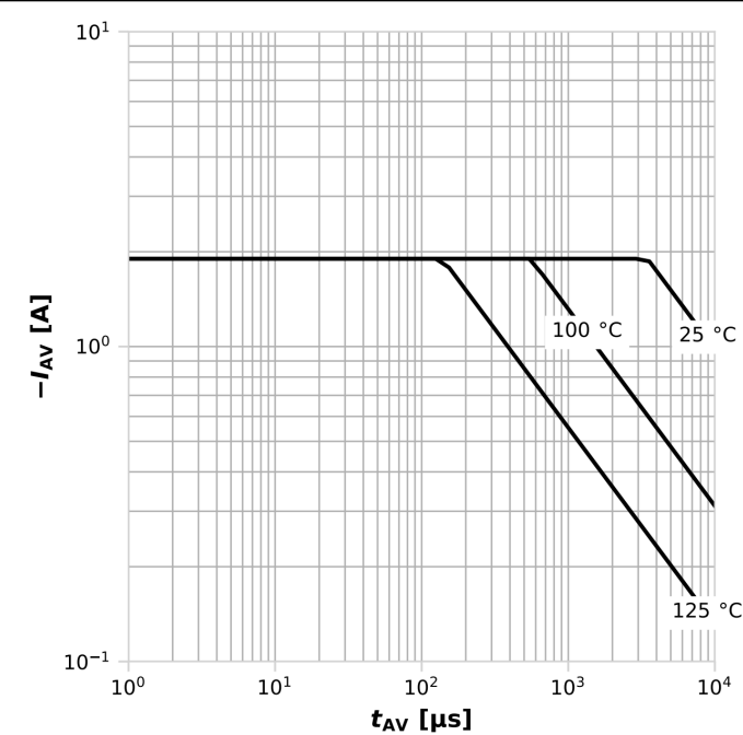
Diagram 13: Avalanche characteristics
