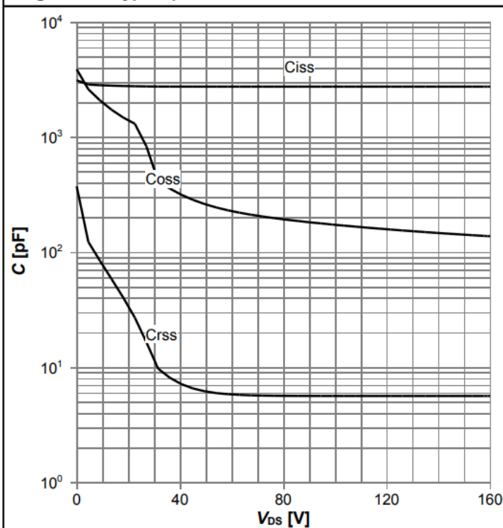
Diagram 11: Typ. capacitances
