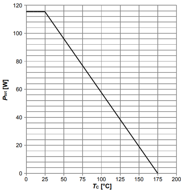
Diagram 1: Power dissipation
