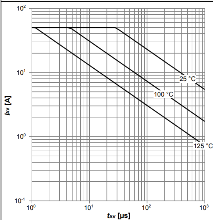
Diagram 13: Avalanche characteristics
