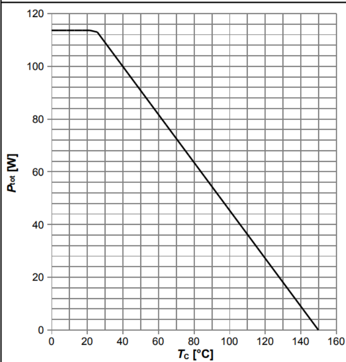
Diagram 1: Power dissipation
