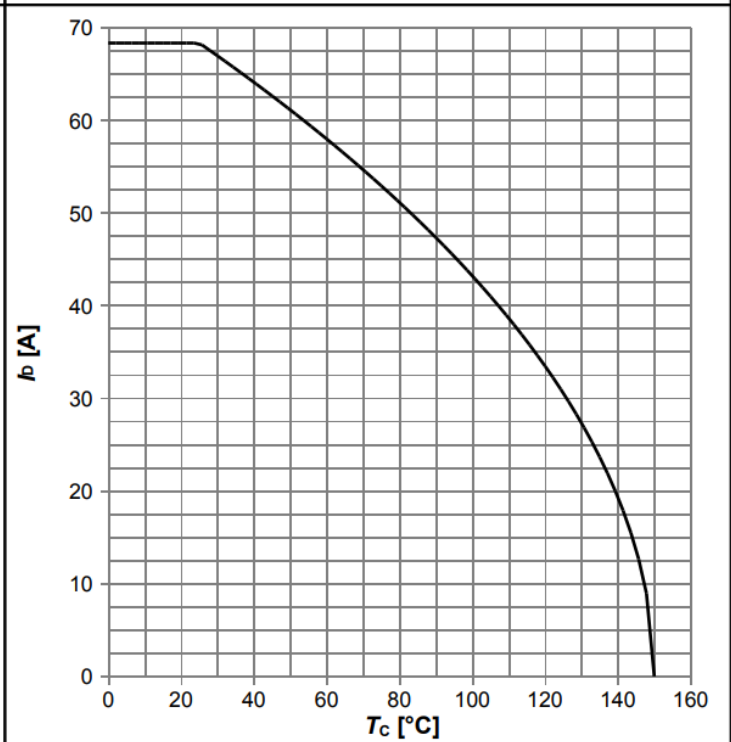
Diagram 2: Drain current
