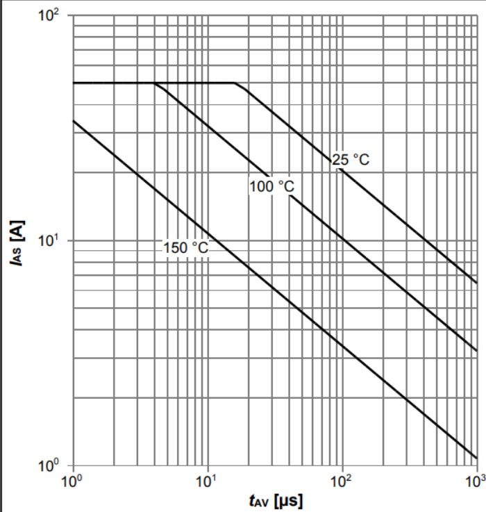
Diagram 13: Avalanche characteristics
