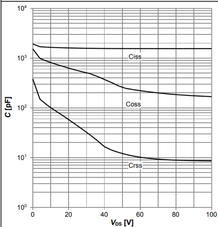
Diagram 11: Typ. capacitances
