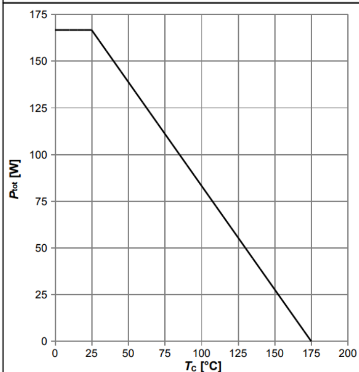
Diagram 1: Power dissipation
