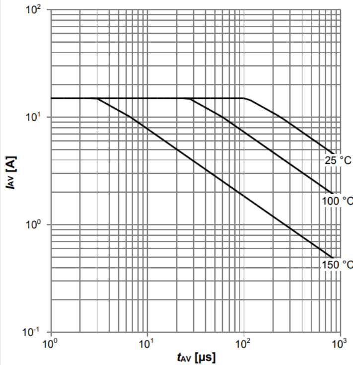
Diagram 13: Avalanche characteristics
